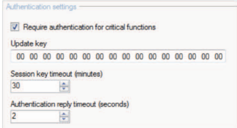
Figure 4: DNP3 Secure Authentication using dynamic keys that are updated, automatically and periodically between a DNP3 Master and Outstation RTU.
