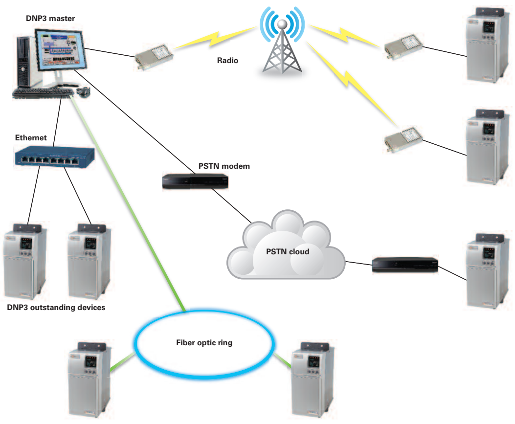
Figure 2: An example multi-layered Telemetry System
